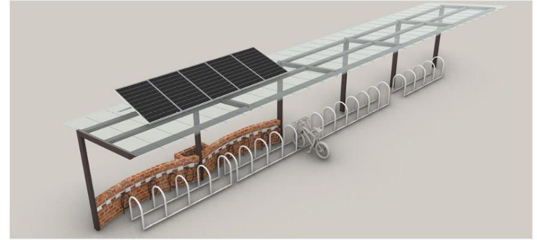
Rendering of potential design using brick masonry
